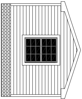
HITCH ELEVATION JPR-EXT-004 #2 AND #3 ONLY
